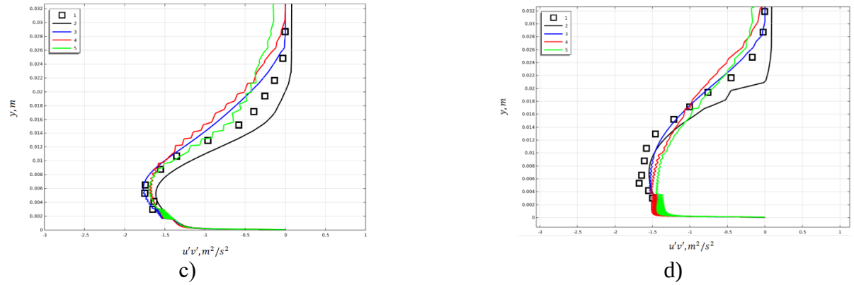
Fig. 7. Profiles of turbulent stresses on the lower surfaces at x = 0.03 a), 0.183 b), 0.335 c), 0.635 d) 1-experiment, 2-two-fluid model, 3-SST model, 4-SA model, 5-v2-f model.
