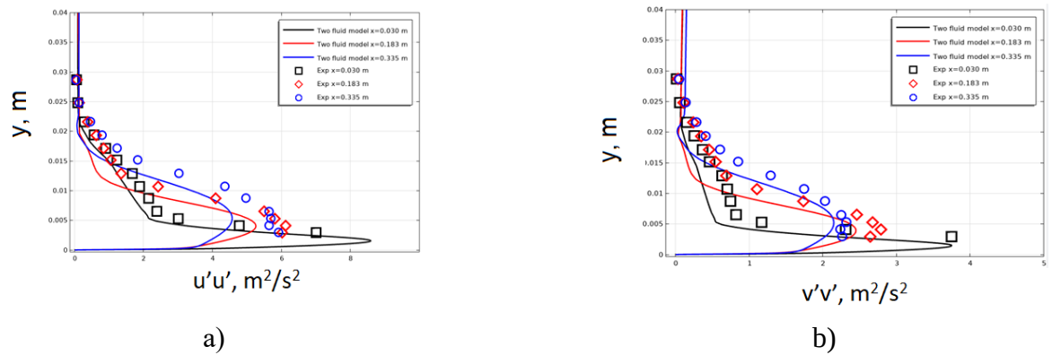
Fig. 8. Profiles of turbulent stresses on the lower surfaces at a) \overline{u'u'} and b) \overline{v'v'} .
