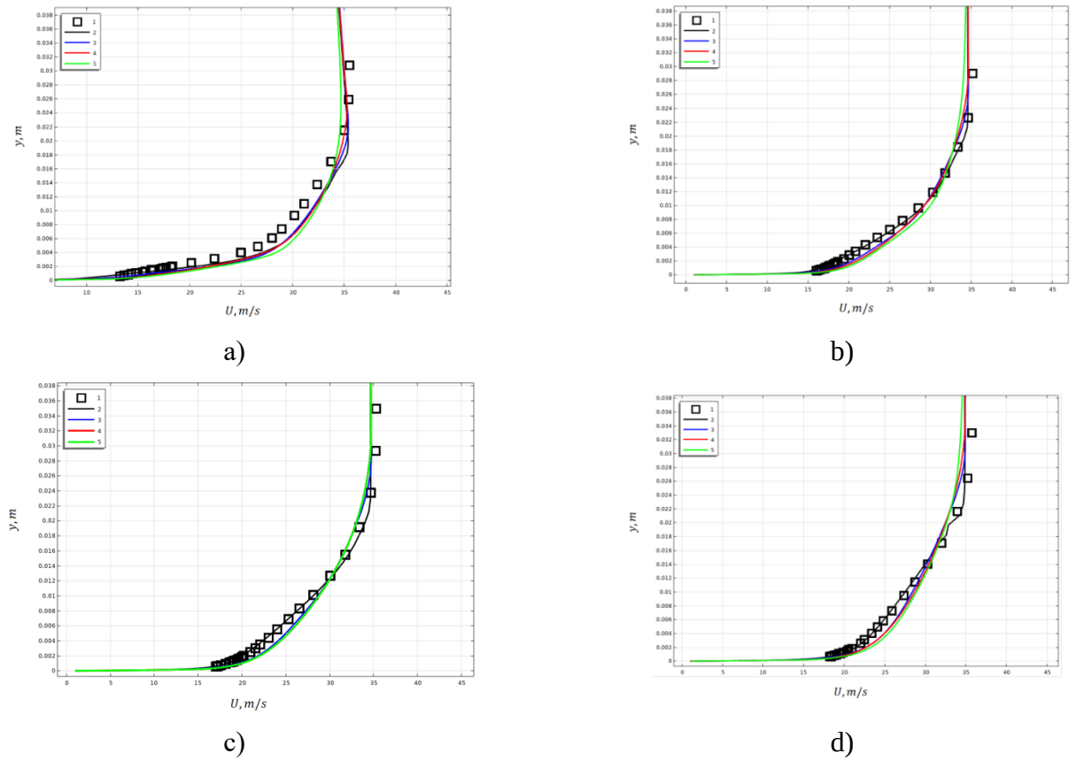
Fig. 6. Longitudinal velocity profiles on the lower surface at x = 0.03 a), 0.183 b), 0.335 c), 0.635 d) 1-experiment, 2-two-fluid model, 3-SST model, 4-SA model, 5- v_2 -f model.
